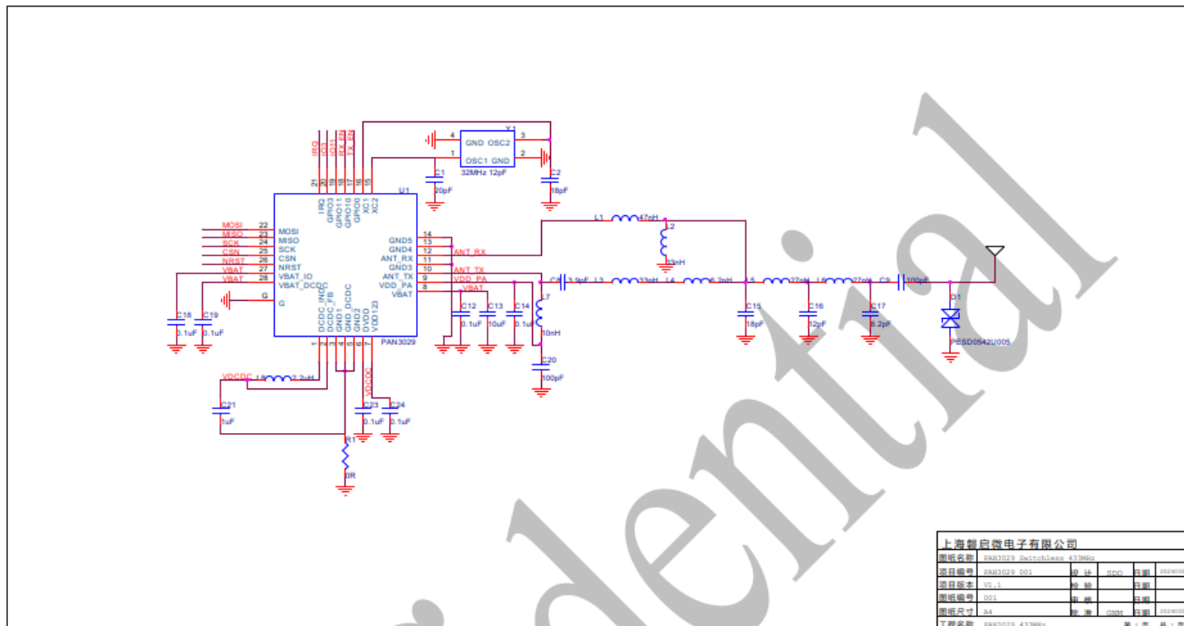
Figure 1-2 433MHz switchless reference schematic
